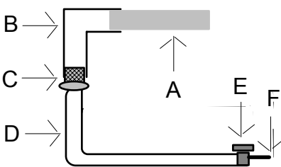
Adapter for Vacuum Packing
