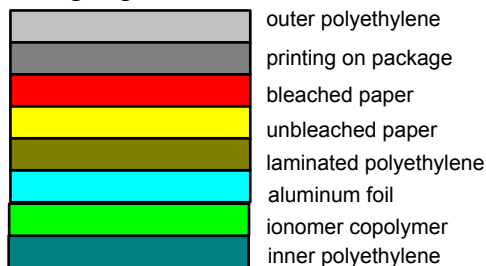
Paperboard Carton Layers
